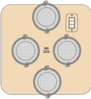
Hearth Infrared Sauna Panel 23.75 x 23.5 x 9 in (60.3 x 59.7 x 22.9 cm)
