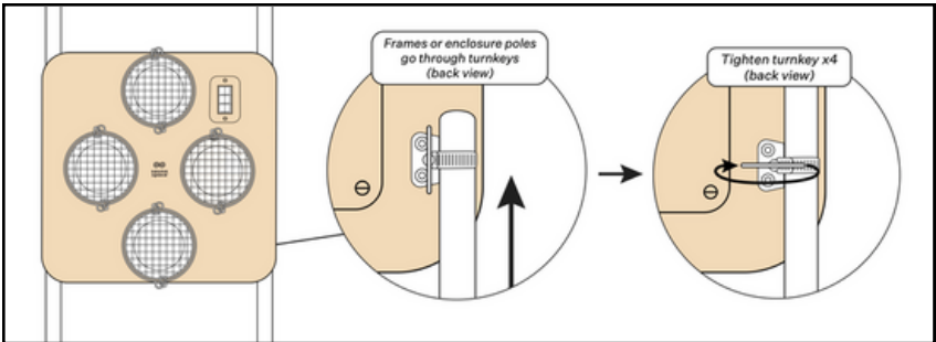
Method 3: Attach to a frame or enclosure
