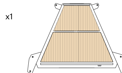
Bamboo grounding mat 49.325 x 48.125 x 22.75 in (125 x 122 x 58 cm) front width x depth x rear width
